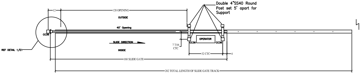
PLAN VIEW SLIDE GATE IN CLOSED POSITION SCALE: 3/4" = 1'-0"
