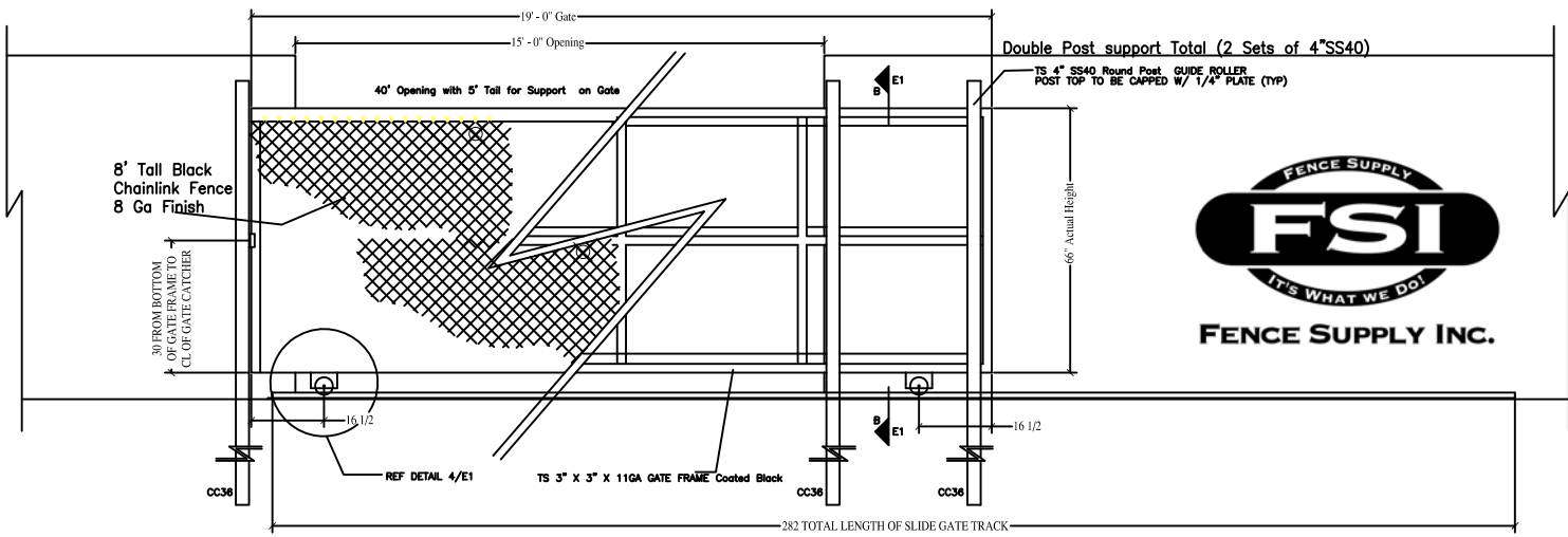
A-A ELEVATION Side Gate SCALE: 3/4" = 1'-0" INSIDE LOOKING OUT
