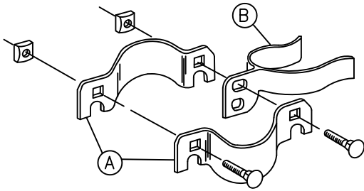
DROP FORK LATCH
