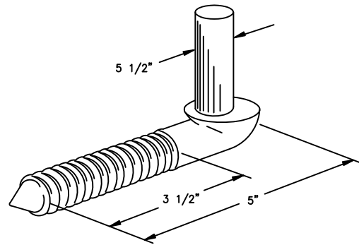
LAG SCREW - MALE HINGE WITH SHOULDER
