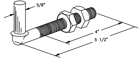
J-BOLT - MALE HINGE WITH TWO BOLTS
