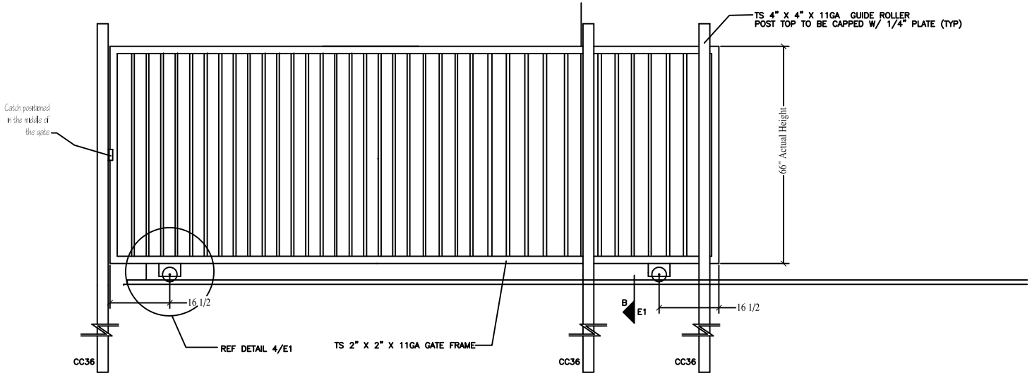
A-A ELEVATION Slide Gate SCALE: 3/4" = 1'-0" INSIDE LOOKING OUT
